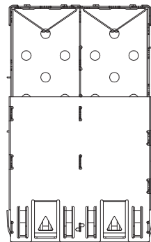
VIEW A
