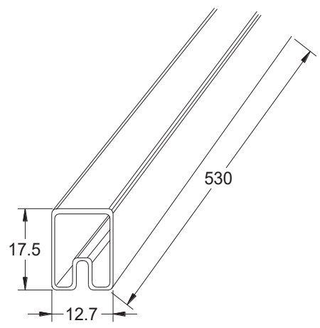
Tube: 530*12.7*17.5mm
