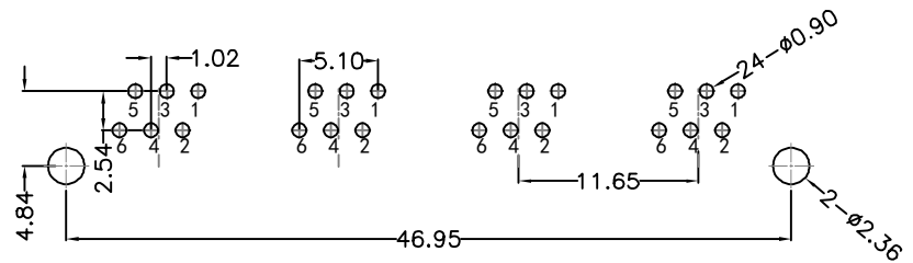
RECOMMENDED PCB LAYOUT VIEWED FROM COMPONENT SIDE
