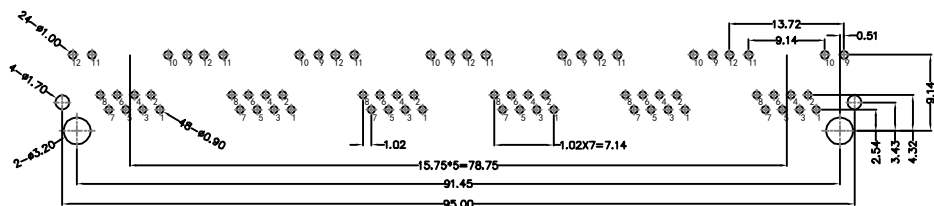
RECOMMENDED PCB LAYOUT VIEWED FROM COMPONENT SIDE
