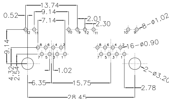
RECOMMENDED PCB LAYOUT VIEWED FROM COMPONENT SIDE
