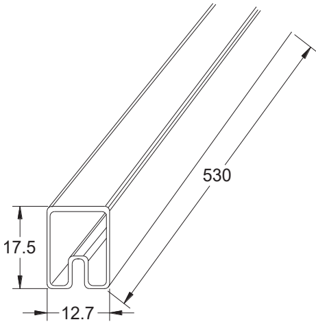
Tube: 530*17.5*12.7mm
