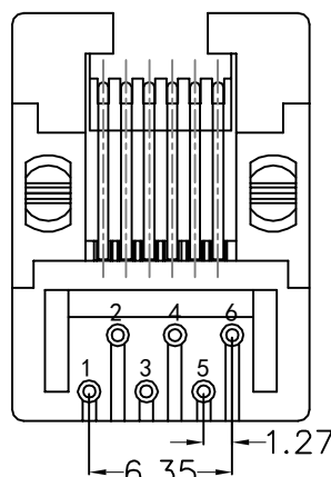
BOTTOM VIEW
