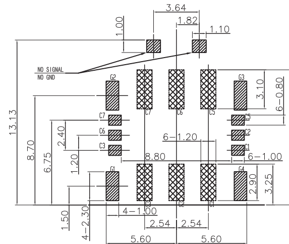
Recommended PCB Layout Top View (Tolerance \pm 0.05 )
