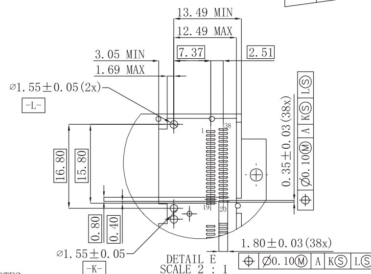
PCB PORT LAYOUT COMPONENT PORT
