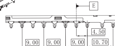
DETAIL C SCALE 2 : 1
