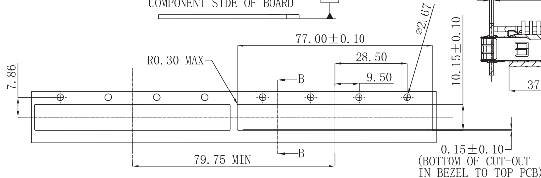
PCB LAYOUT FOR SINGLE SIDED APPLICATION
